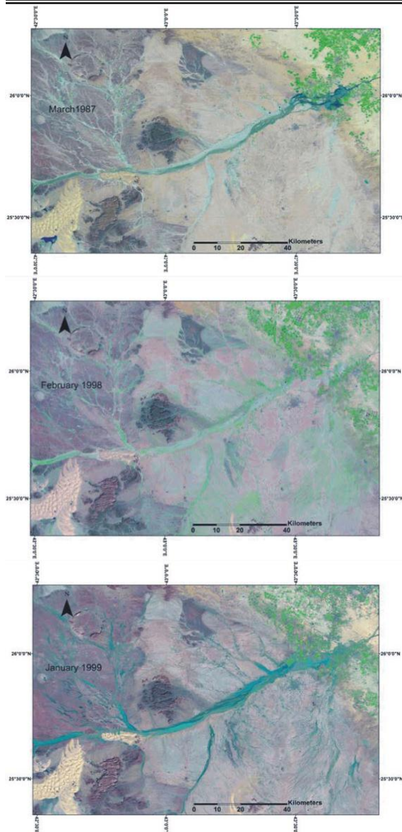
Fig. 3: Distribution and extent of active channels and flash floods based on the Landsat images, March 1987 (top), February 1998 (middle) and January 1999 (bottom)
