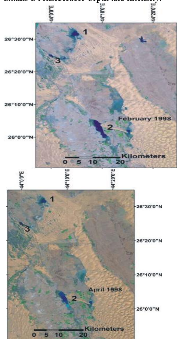
Fig. 6 : The resultant water ponds of the flash flood of January 1998 (Note: the changes of surface extent between February and April 1998. The stored water volumes in ponds 1, 2 and 3 were computed using these delineated surface areas and the dry-bottom topography derived from the SRTM)
