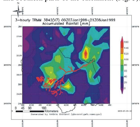
Fig. 5 A: TRMM estimated total rainfall(mm) and distribution over Wadi Al Rimah catchment on the 7 th of January 1999. Note: the correspondence between the rainfall pattern and the resulting active channels (red lines), which are digitized from the Landsat image acquired shortly after this rainfall event (Fig. 3)
