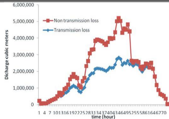
Fig.7: The simulated runoff hydrograph for Wadi Al Rimah using the entire flow contributing areas (i.e. time zones) and the distributed rainfall of Fig. 5 A. (Note :the impact of transmission loss on the hydrograph peaks and attenuations).
