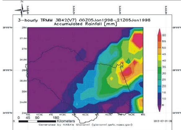
Fig. 5 B: TRMM data of the 5 th of January rainfall event Note the considerable differences in rainfall patterns each event
