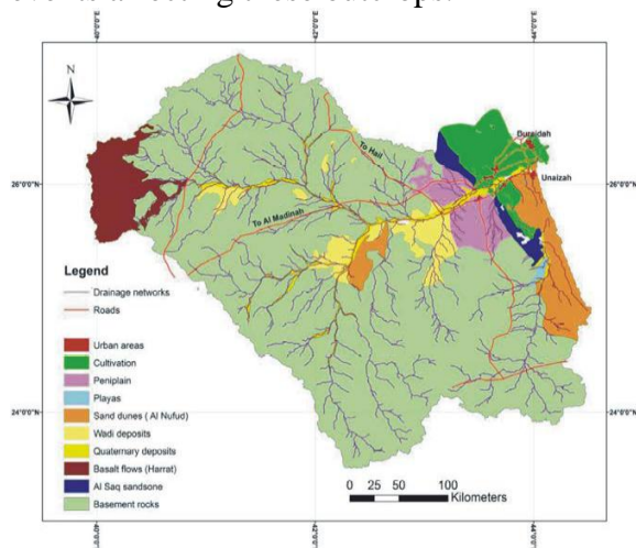
Fig. 2 : The land cover map of Wadi Al Rimah, based on the geological maps ‘DEM and Landsat TM image of 1999
